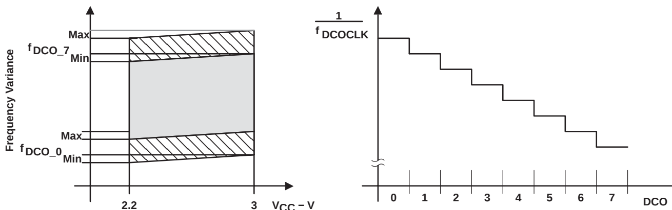
Figure 12. DCO Characteristics
