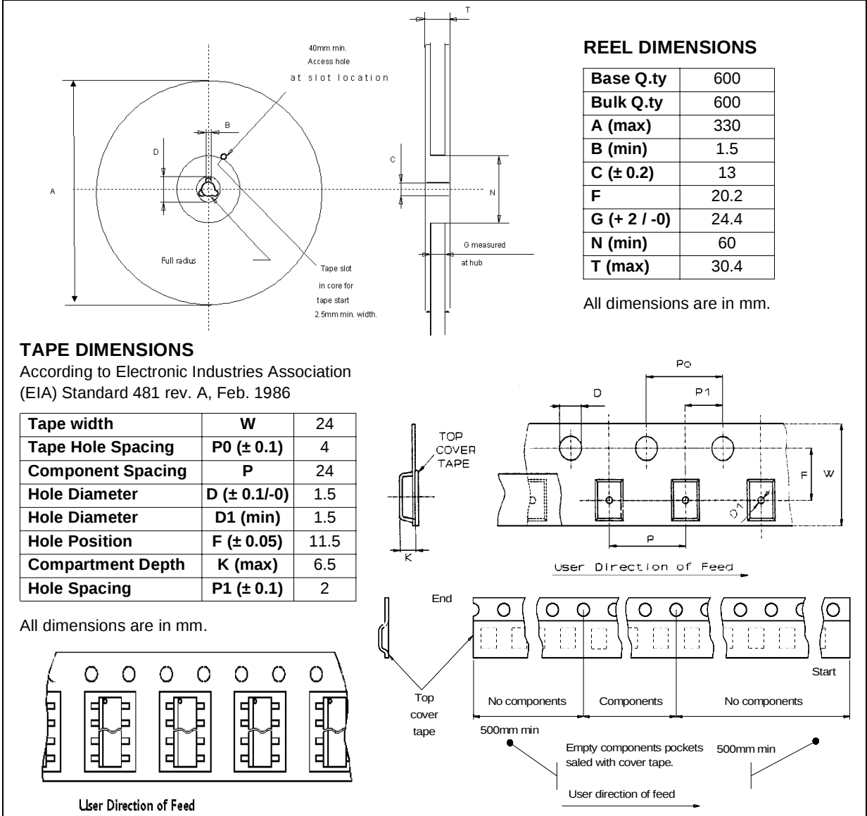
Figure 14. Tape And Reel Shipment (suffix “TR”)
