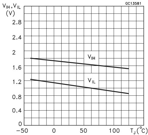
Figure 12. Input voltages vs Junction Temperature
