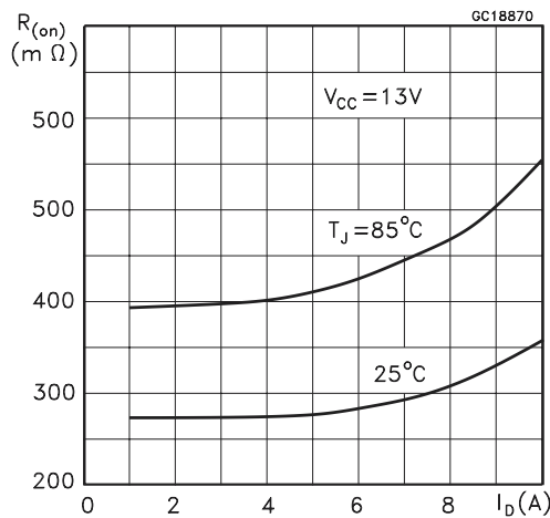
Figure 11. R_{DS(on)} vs Output Current
