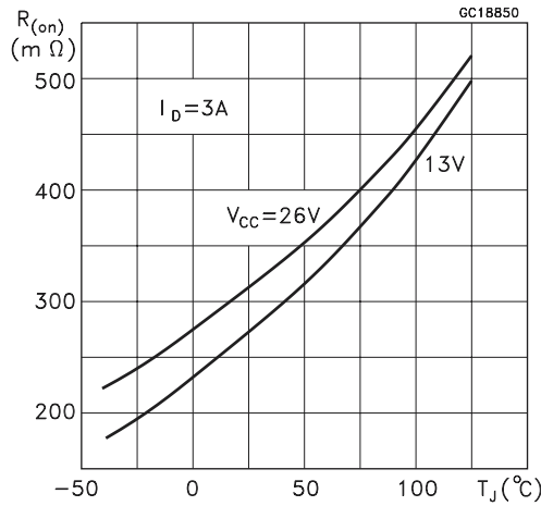
Figure 9. R_{DS(on)} vs Junction Temperature
