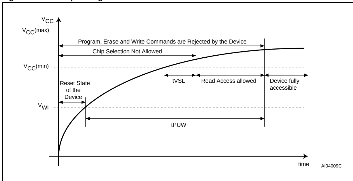
Figure 20. Power-up Timing
