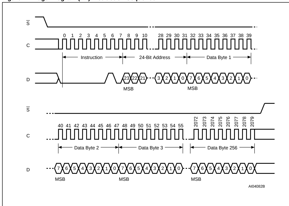
Figure 14. Page Program (PP) Instruction Sequence
