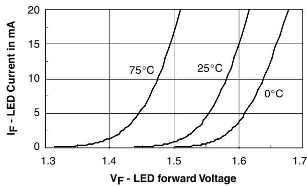
Figure 3. LED forward current vs. forward voltage
