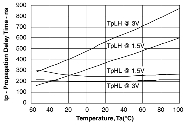
Figure 8. Propagation Delay vs. Temperature-SFH6316T and SFH6343T
