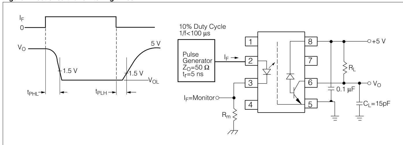
Figure 1. Test circuit for switching times
