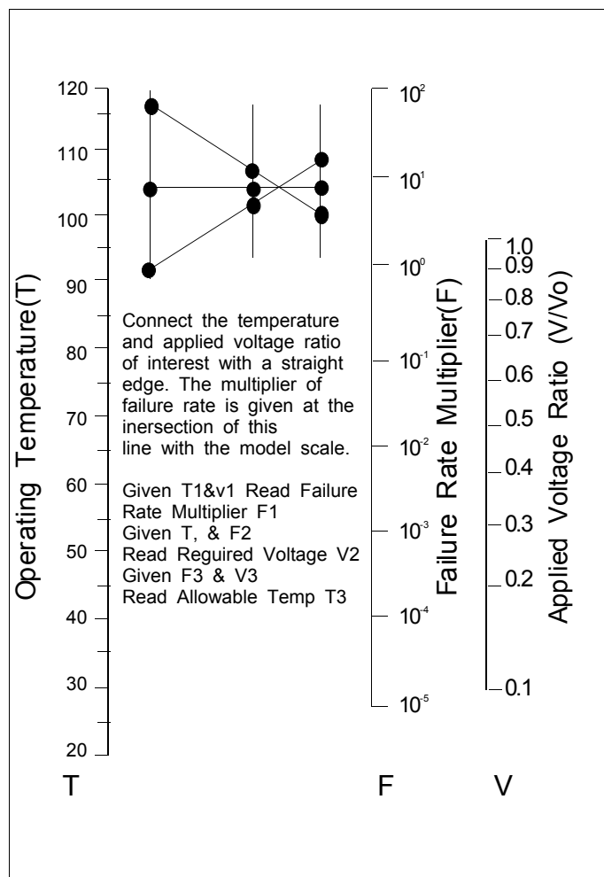
Fig.8 Reliability Nomograph
