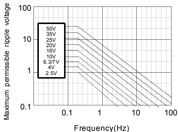
Fig.7 Maximum permissible ripple voltage (C,D)
