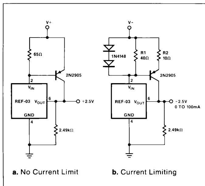
FIGURE 5: Output Current Boost
