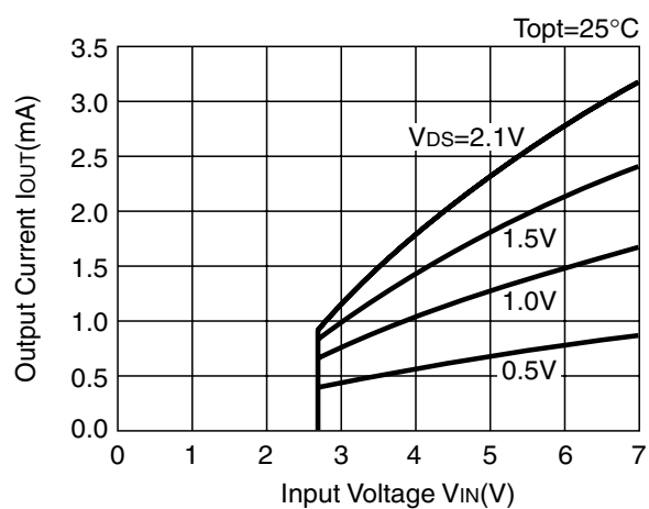
R3111x27xC
