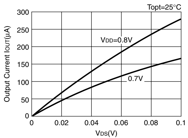
R3111x27xC
