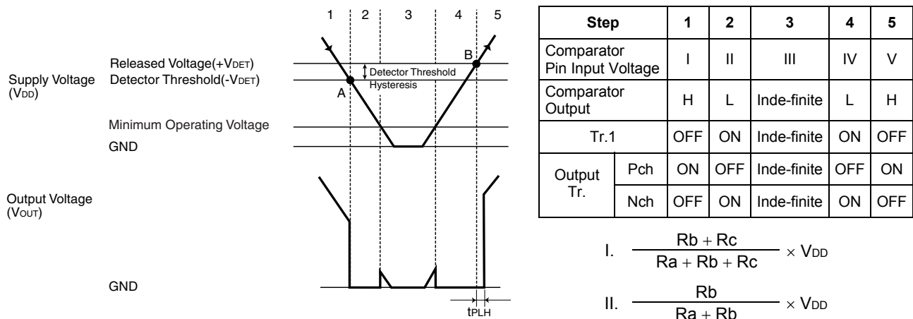
Figure 2. Operation Diagram
