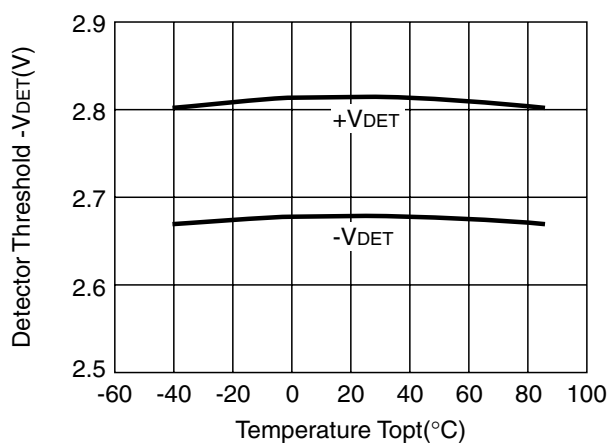
R3111x27xC
