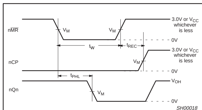
Waveform 2. Master Reset ( \overline{\text{MR}} ) Pulse Width, \overline{\text{MR}} to Output propagation Delay and \overline{\text{MR}} to Clock Recovery Time
