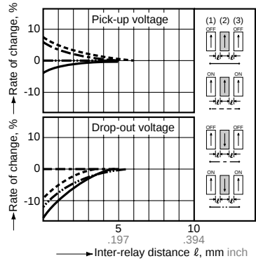
6-(2). Influence of adjacent mounting (2 Form C)
