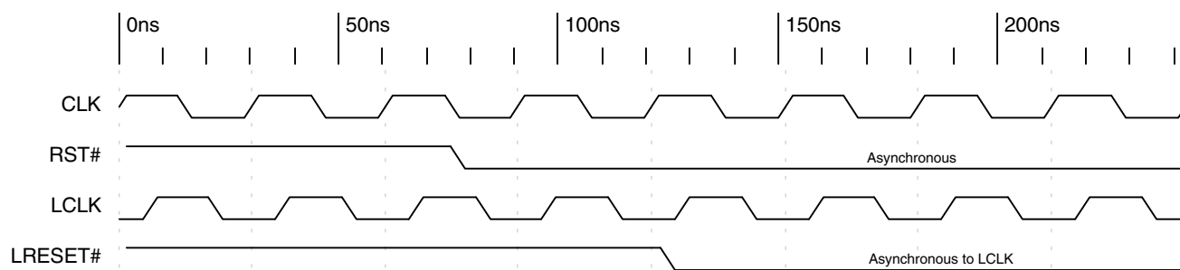
Timing Diagram 4-2. PCI RST# Asserting Local Output LRESET#
