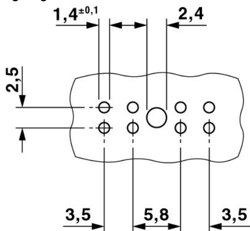
Drilling diagram
