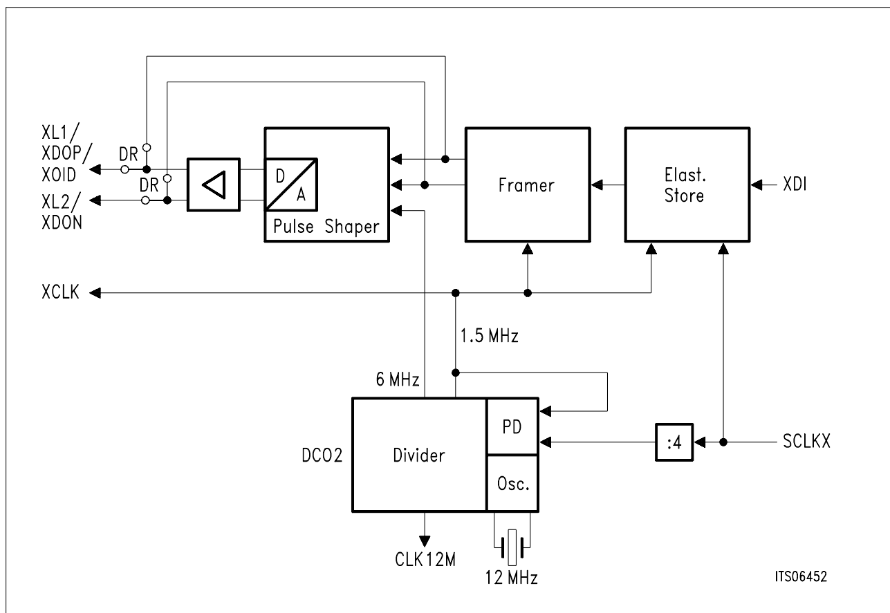
Figure 45 Transmit Clock System
