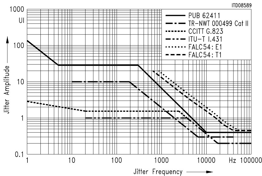
Figure 44 Jitter Tolerance
