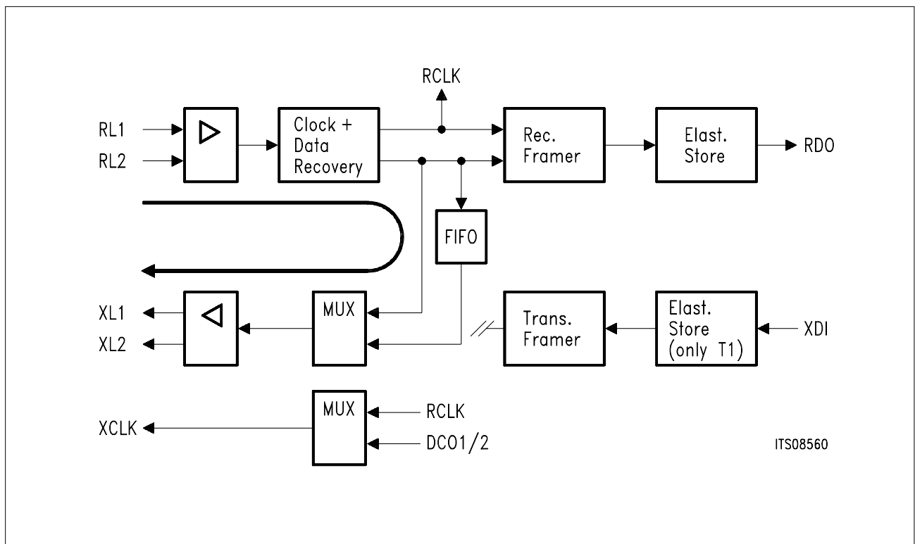
Figure 20 Remote Loop
