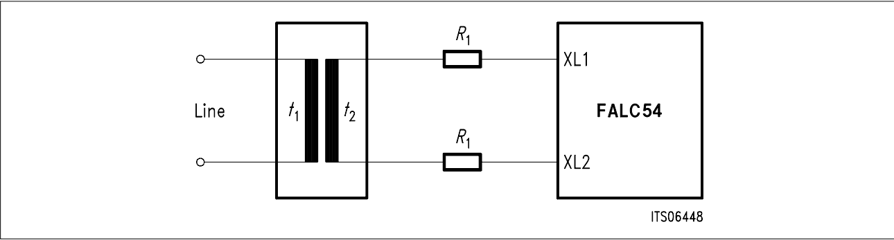
Figure 15 Transmitter Configuration
