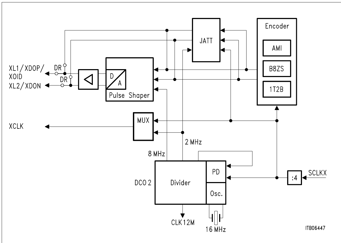
Figure 13 Transmit Clock System
