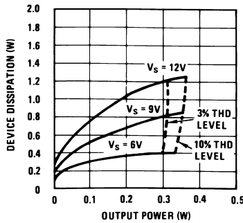
Device Dissipation vs Output Power — 4 \Omega Load
