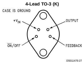
Bottom View LM1575K-XX or LM1575HVK-XX/883 See NS Package Number K04A
