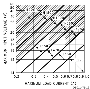
FIGURE 5. LM2575(HV)-12
