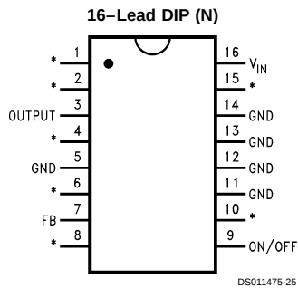
Top View LM2575N-XX or LM2575HVN-XX See NS Package Number N16A
