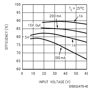
Efficiency
