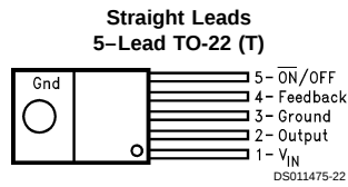
Top View LM2575T-XX or LM2575HVT-XX See NS Package Number T05A
