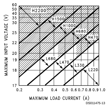
FIGURE 6. LM2575(HV)-15
