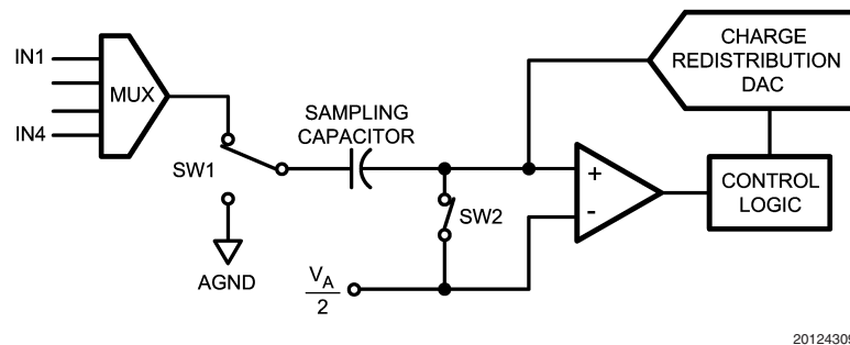
FIGURE 1. ADC124S021 in Track Mode
