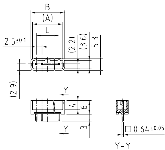
Straight plug
