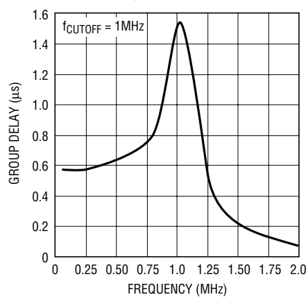
Group Delay
