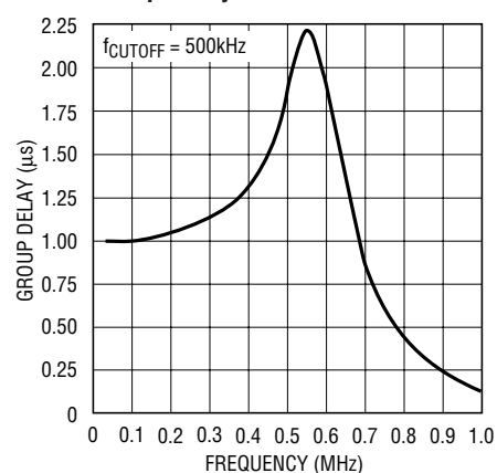
Group Delay
