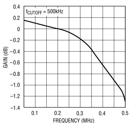
Passband Gain
