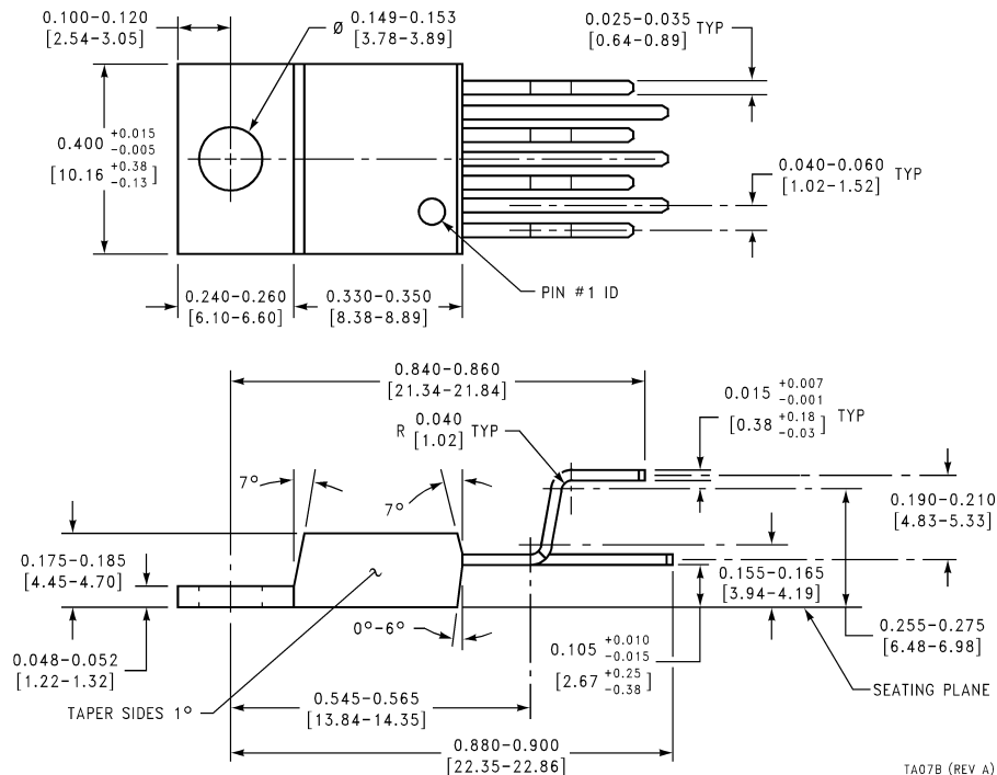
TO-220 Power Package Order Number LM2676T-3.3, LM2676T-5.0, LM2676T-12 or LM2676T-ADJ NS Package Number TA07B
