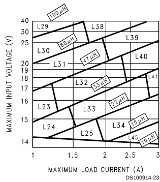
FIGURE 5. LM2676-12
