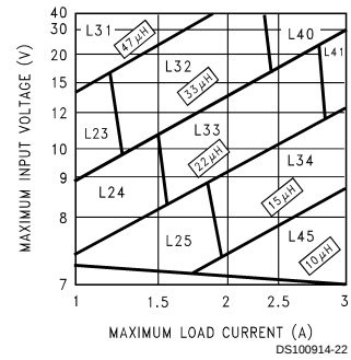
FIGURE 4. LM2676-5.0
