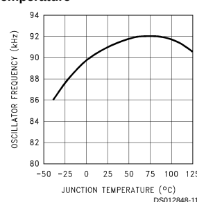
Oscillator Frequency vs Junction Temperature
