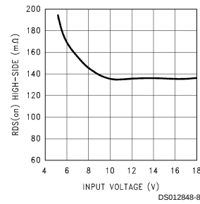
R_{DS(on)} High-Side vs Input Voltage
