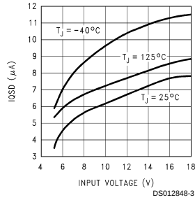
I_{QSD} vs Input Voltage
