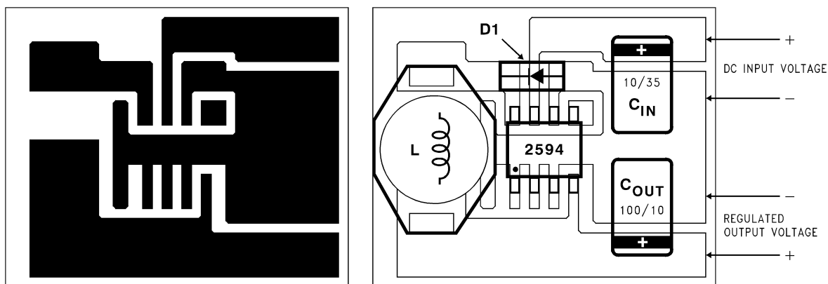
TYPICAL SURFACE MOUNT PC BOARD LAYOUT, FIXED OUTPUT (2X SIZE)
