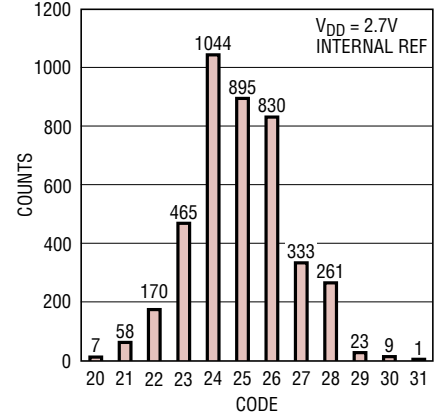
Histogram for 4096 Conversions (LTC1867L)
