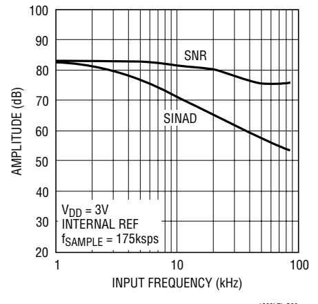
Signal-to-(Noise + Distortion) Ratio vs Input Frequency
