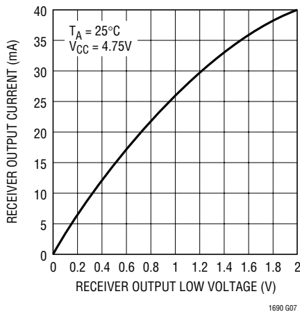
Receiver Output Low Voltage vs Output Current
