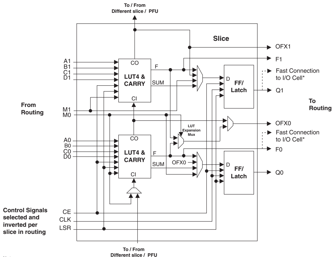
Figure 2-5. Slice Diagram
