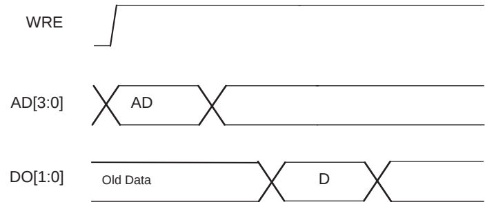
Figure 3-6. Slice Single/Dual Port Read Cycle Timing
