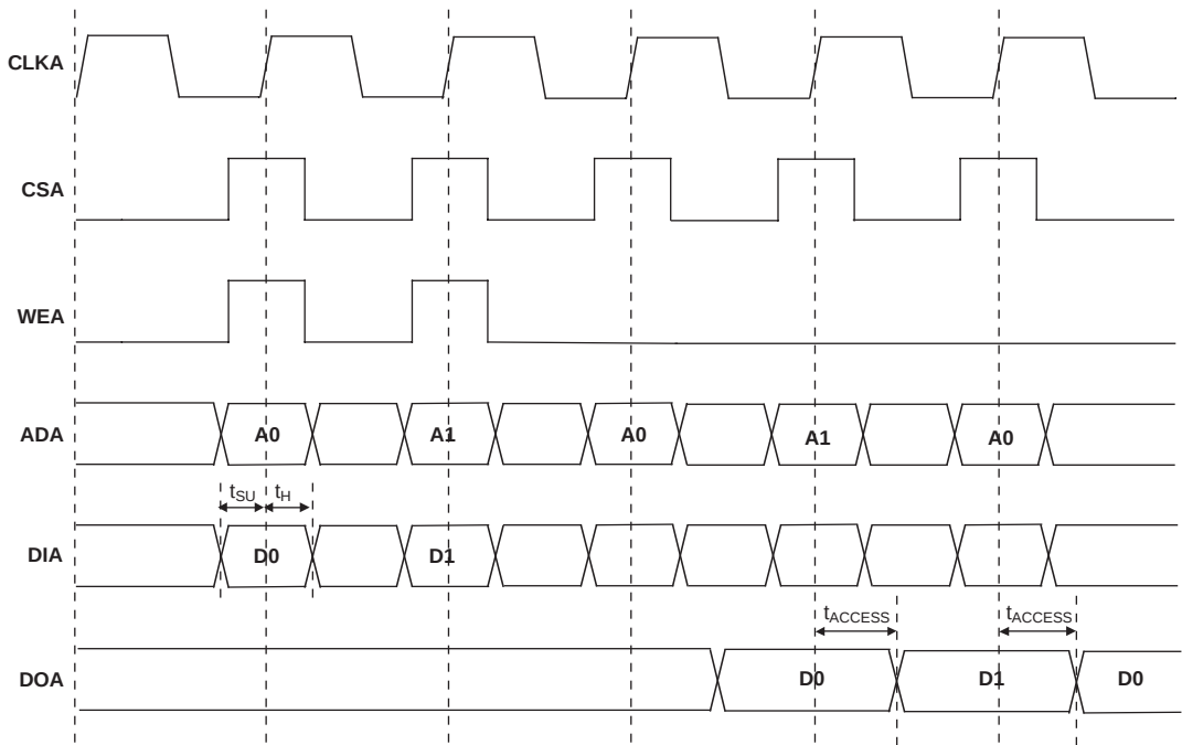
Figure 3-7. Read Mode (Normal)
