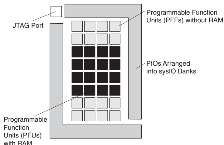
Figure 2-3. Top View of MachXO256 Device
