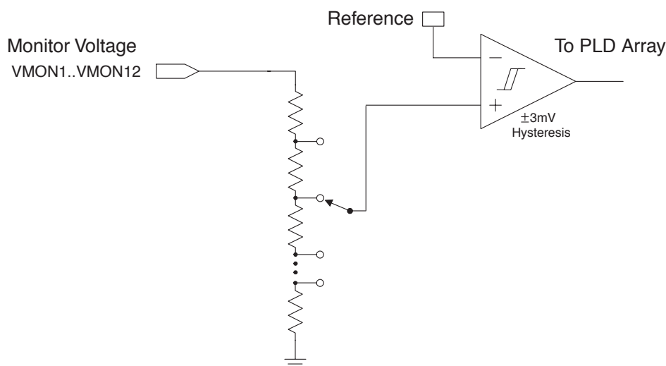
Figure 2. Voltage Monitors
