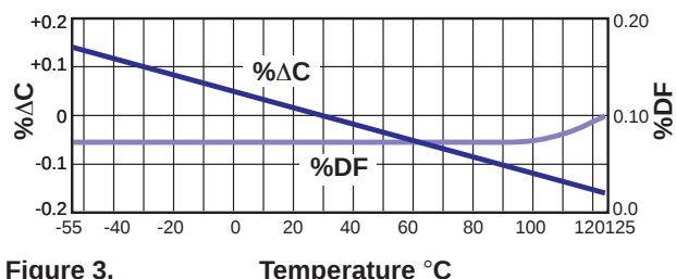
Figure 3. Temperature °C Capacitance & DF vs Temperature - C0G
