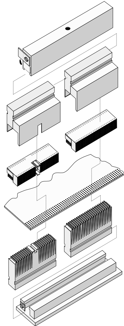
Modular press-fit tool for female connector modules 5+2
