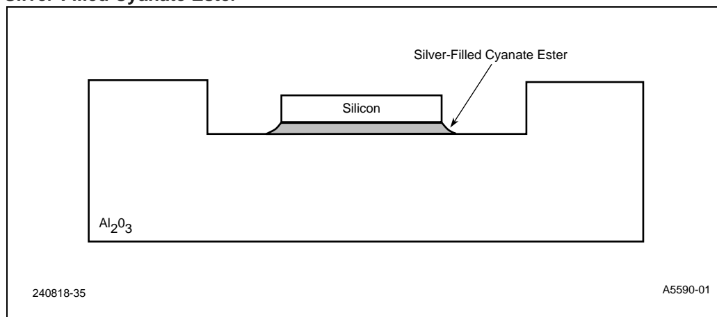
Figure 3-4. Silver-Filled Adhesive
