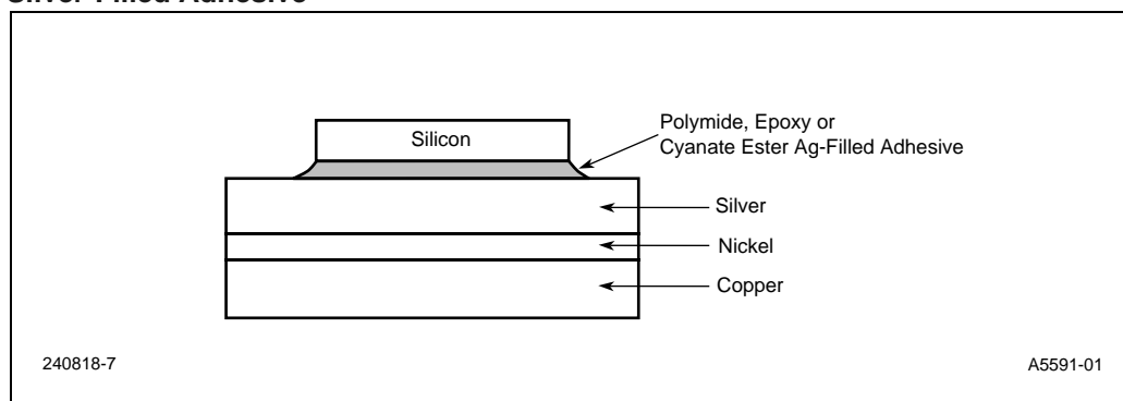
Figure 3-4. Silver-Filled Adhesive
