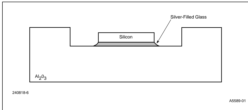
Figure 3-2. Silver-Filled Glass
