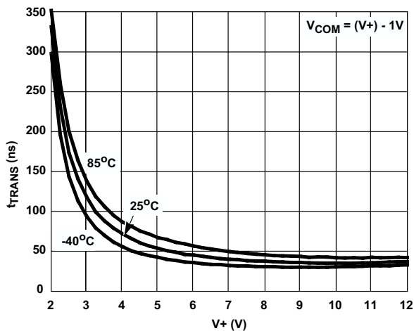
FIGURE 14. ADDRESS TRANS TIME vs SUPPLY VOLTAGE
