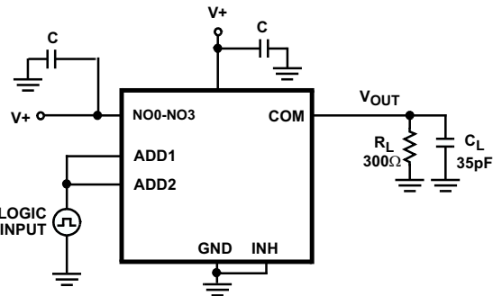
FIGURE 3B. TEST CIRCUIT
