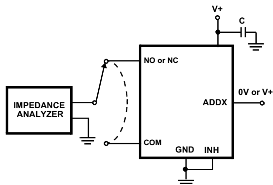
FIGURE 6. CAPACITANCE TEST CIRCUIT
