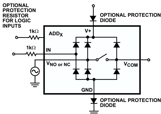
FIGURE 7. OVERVOLTAGE PROTECTION
