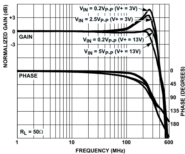
FIGURE 16. FREQUENCY RESPONSE
