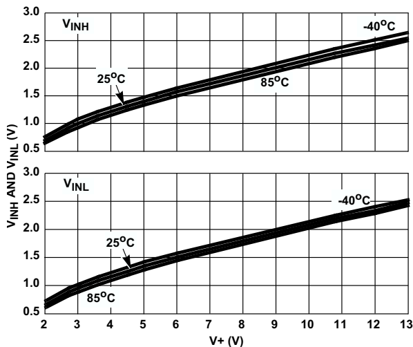
FIGURE 10. DIGITAL SWITCHING POINT vs SUPPLY VOLTAGE
