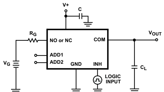
FIGURE 2B. TEST CIRCUIT
