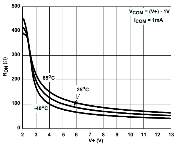
FIGURE 8. ON RESISTANCE vs SUPPLY VOLTAGE
