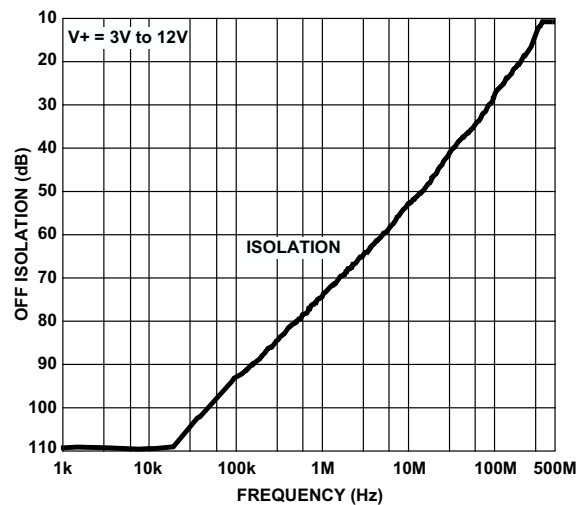
FIGURE 17. OFF ISOLATION
