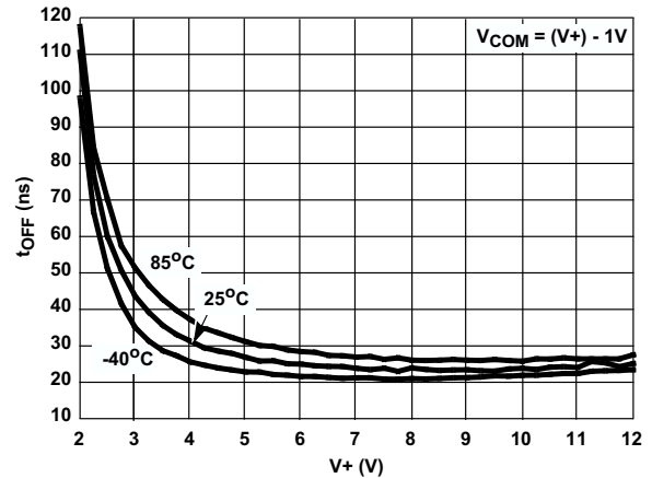
FIGURE 13. TURN - OFF TIME vs SUPPLY VOLTAGE
