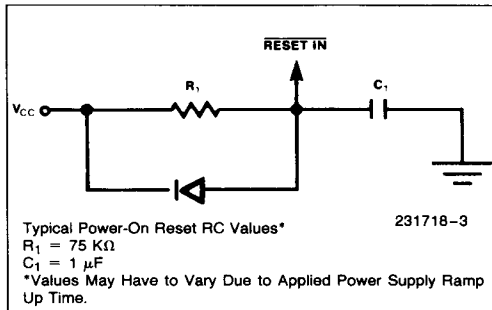
Figure 3. Power-On Reset Circuit
