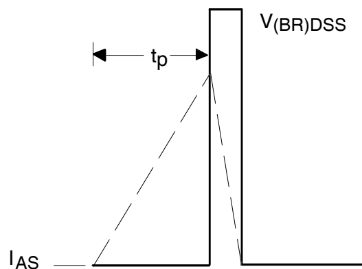
Fig 15b. Unclamped Inductive Waveforms
