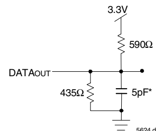
Figure 2. Output Test Load (For t IZ , t HZ , t WZ , t OW ) *Including scope and jig.
