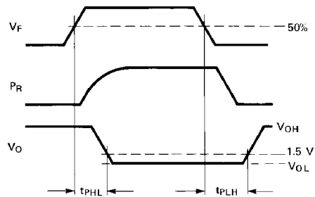
Figure 26. Propagation Delay Test Waveforms.
