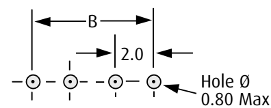
Recommended PC Board Pattern
