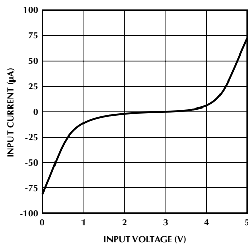
Figure 2. CLK IN Input Current vs. Input Voltage.
