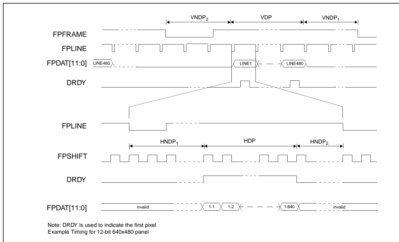
Figure 6-29: 12-Bit TFT Panel Timing
