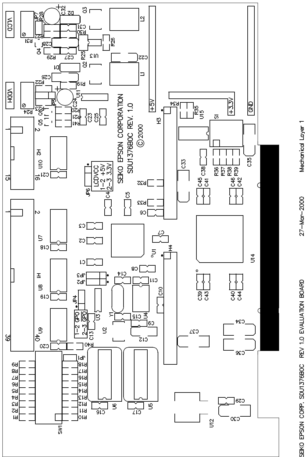
Figure 11-1: S5U13706B00C Board Layout
