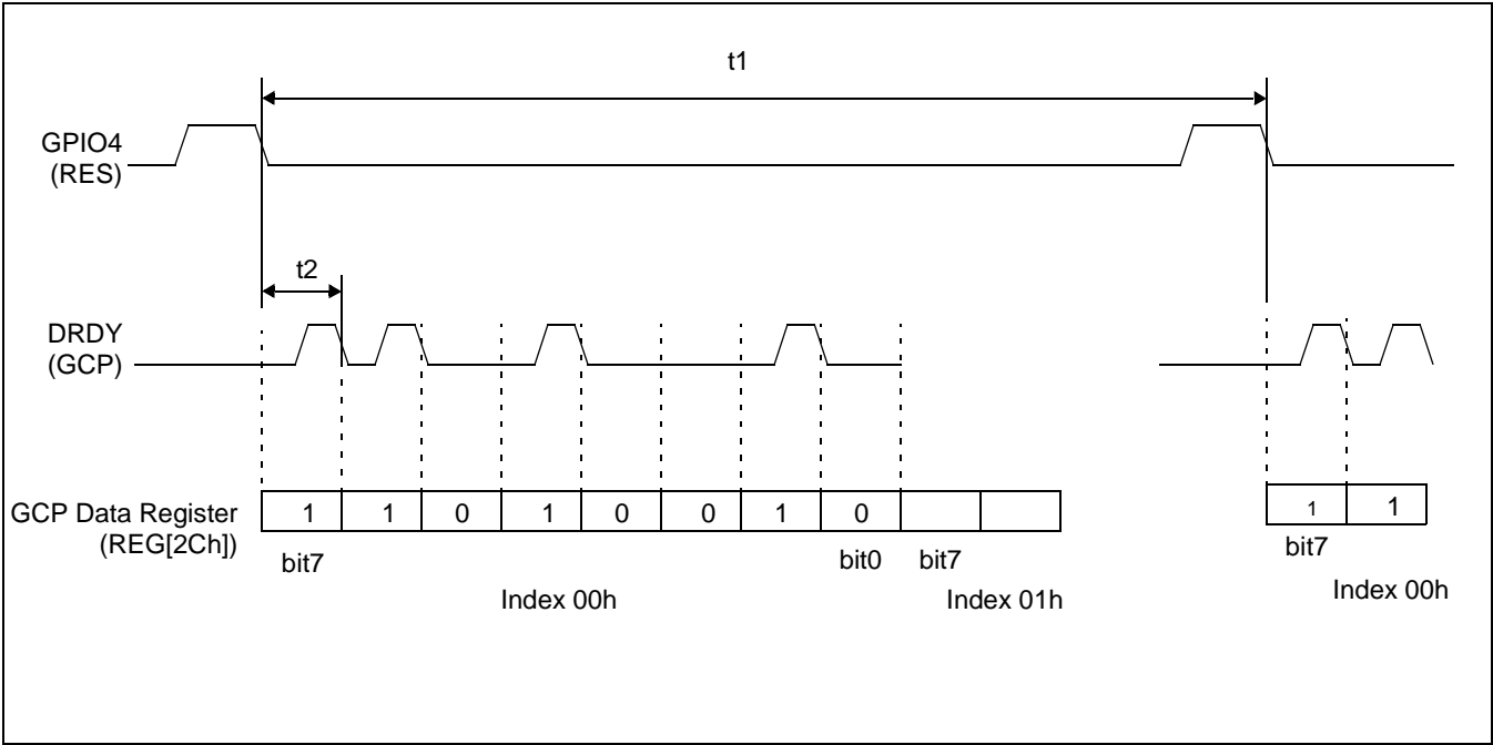
Figure 6-39: 320x240 Epson D-TFD Panel GCP Horizontal Timing
