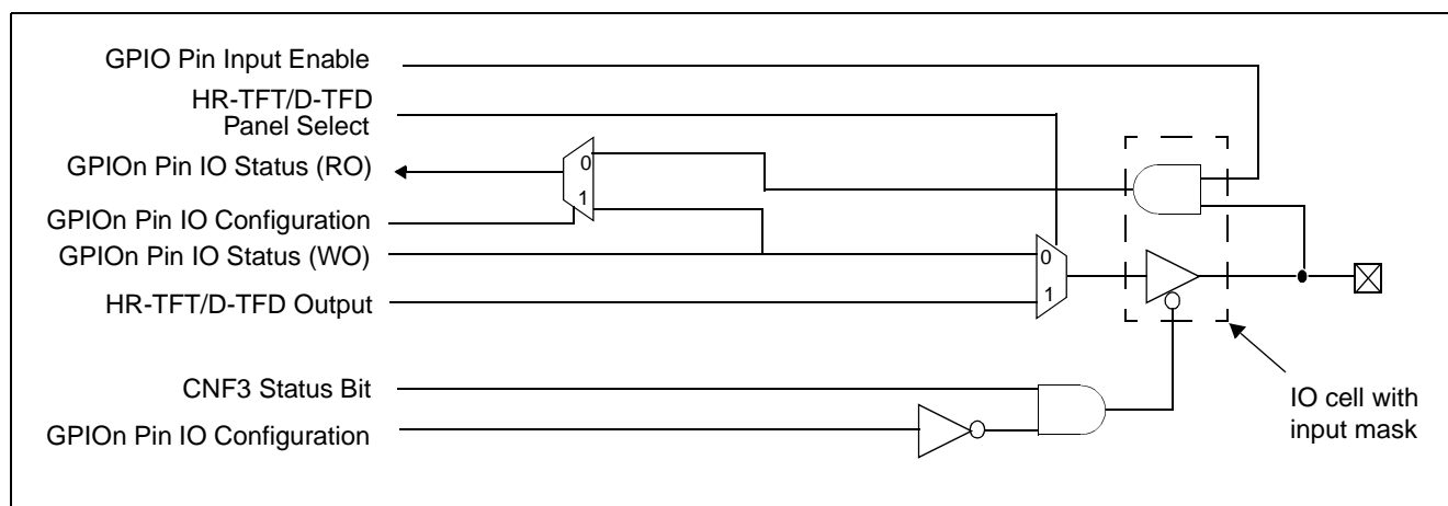
Figure 8-2: Example IO Cell
