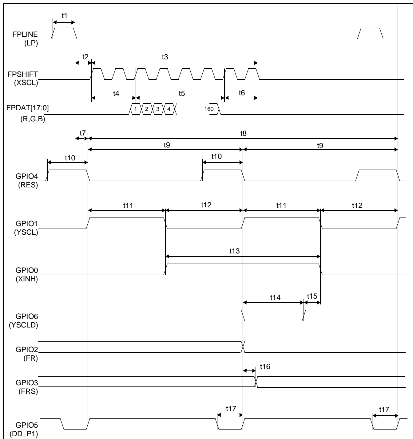
Figure 6-35: 160x240 Epson D-TFD Panel Horizontal Timing
