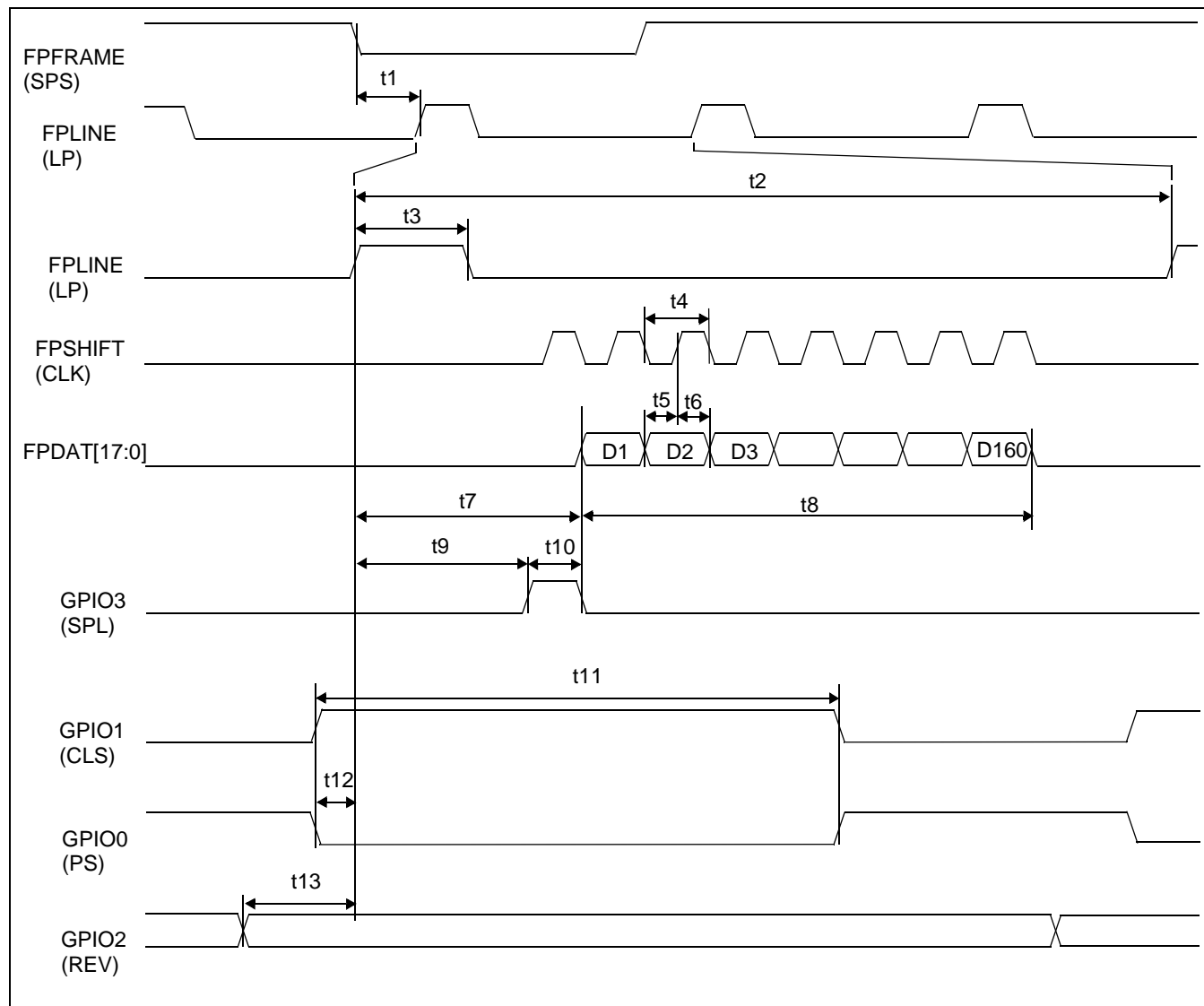
Figure 6-31: 160x160 Sharp HR-TFT Panel Horizontal Timing
