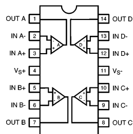
EL2470C SO, P-DIP
