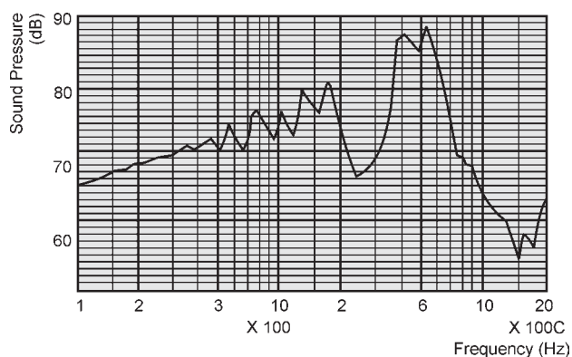
Typischer Frequenzgang Typical frequency response
