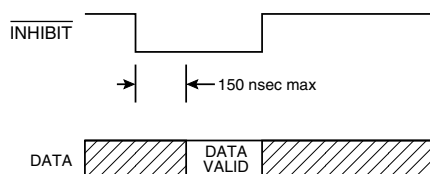
FIGURE 18. INHIBIT TIMING
