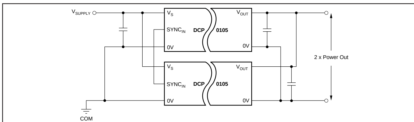
FIGURE 6. Connecting Multiple DCP0105s in Parallel.
