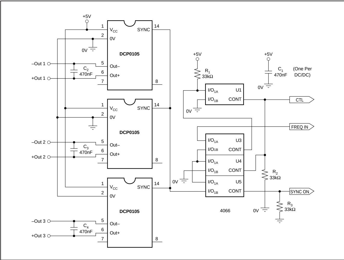
FIGURE 3. Universal Interface.
