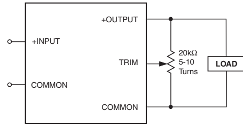
Figure 7. Trim Connections Using a Trimpot
