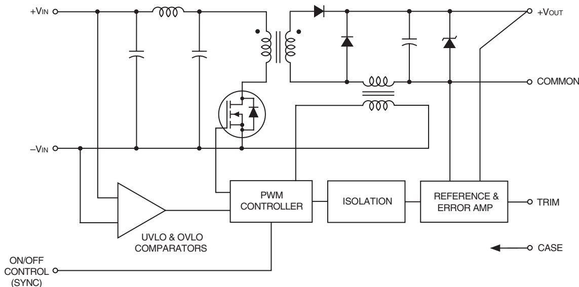
Figure 1. Simplified Schematic
