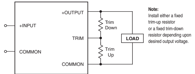
Figure 8. Trim Connections Using Fixed Resistors
