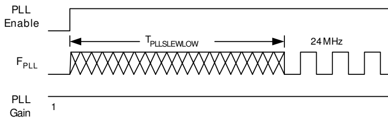
Figure 3-4. PLL Lock for Low Gain Setting Timing Diagram
