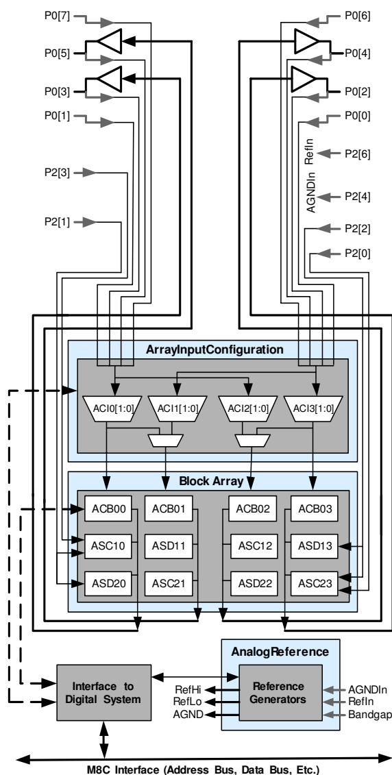
Analog System Block Diagram
