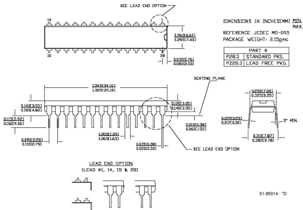
Figure 4-4. 28-Lead (300-Mil) Molded DIP
