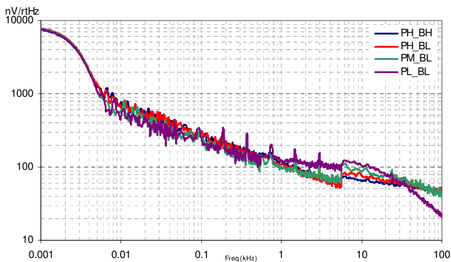
Figure 3-10. Typical Opamp Noise
