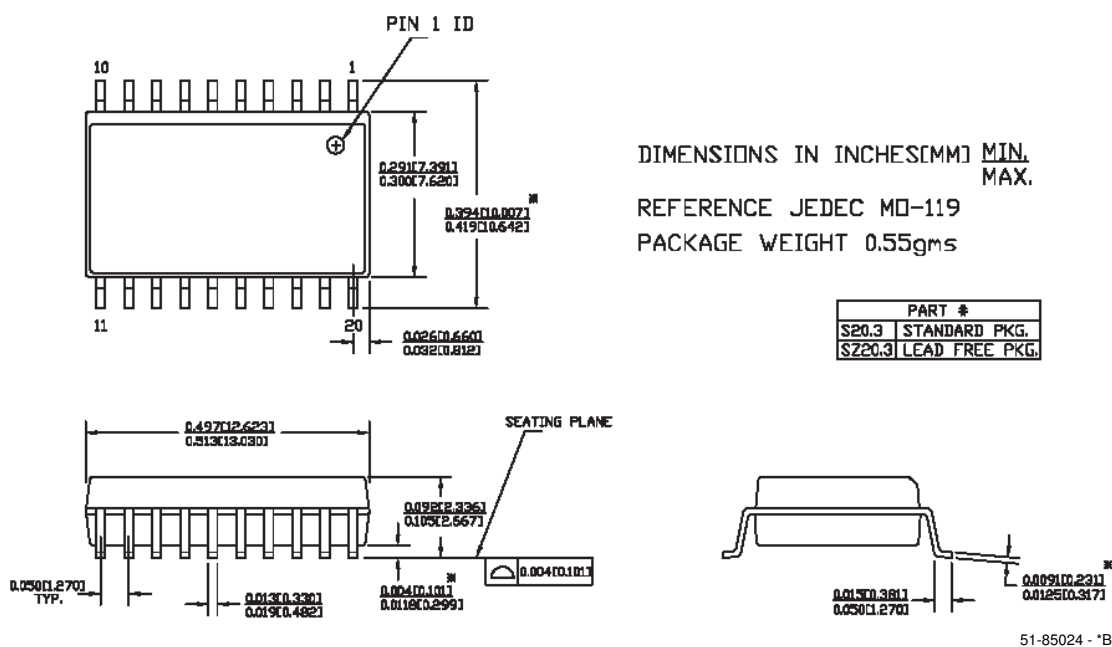
Figure 4-3. 20-Lead (300-Mil) Molded SOIC
