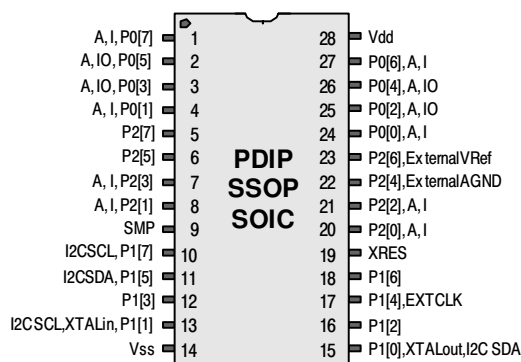
CY8C27443 28-Pin PSoC Device
