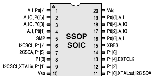
CY8C27243 20-Pin PSoC Device
