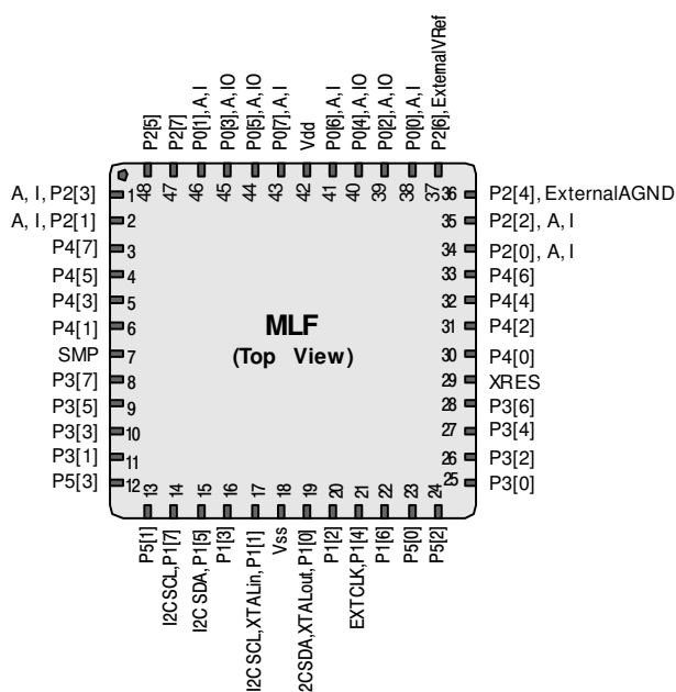
CY8C27643 48-Pin PSoC Device
