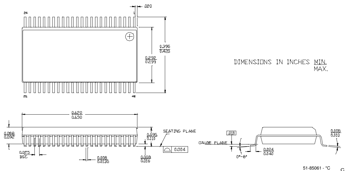
Figure 4-8. 48-Lead (300-Mil) SSOP
