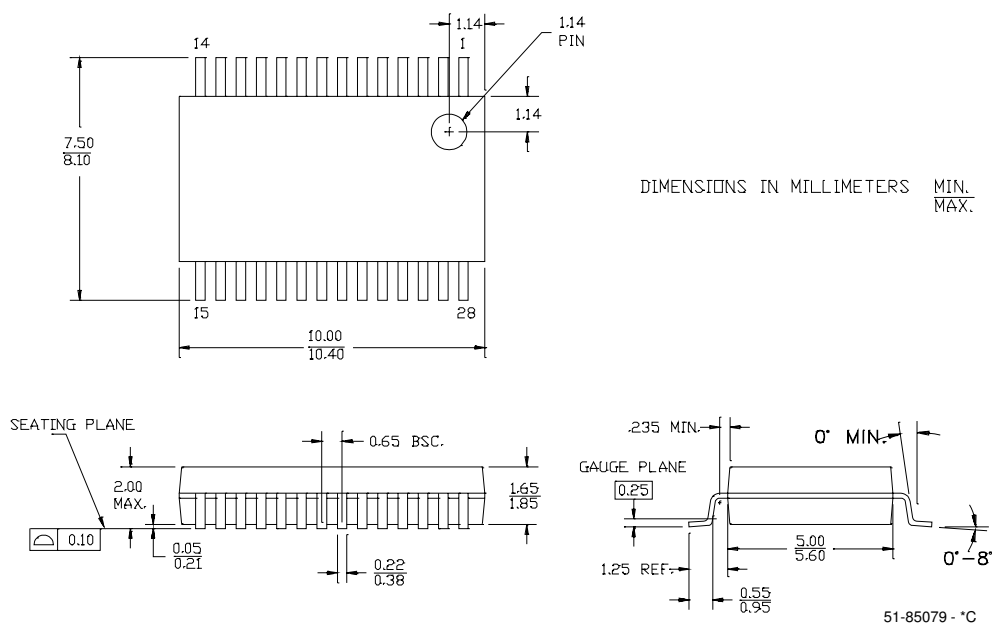
Figure 4-5. 28-Lead (210-Mil) SSOP
