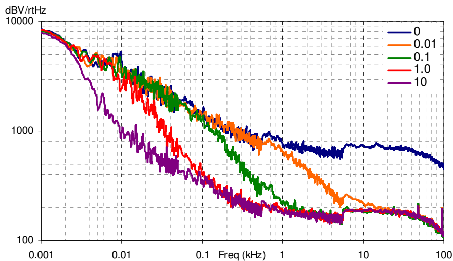
Figure 3-9. Typical AGND Noise with P2[4] Bypass
