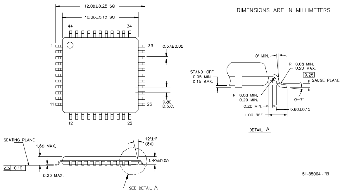
Figure 4-7. 44-Lead TQFP
