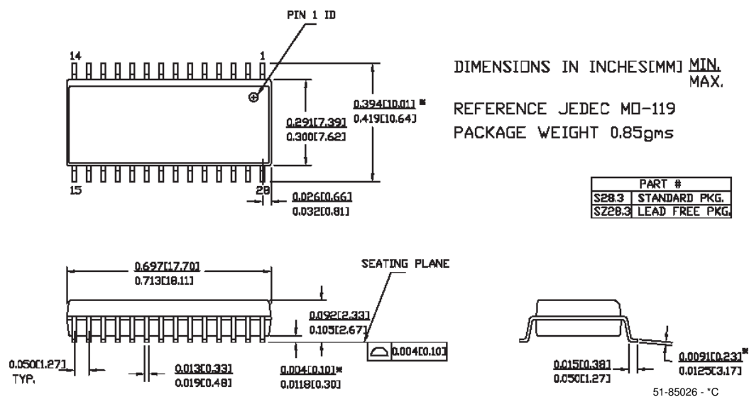
Figure 4-6. 28-Lead (300-Mil) Molded SOIC
