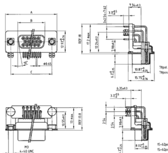
Socket connector
