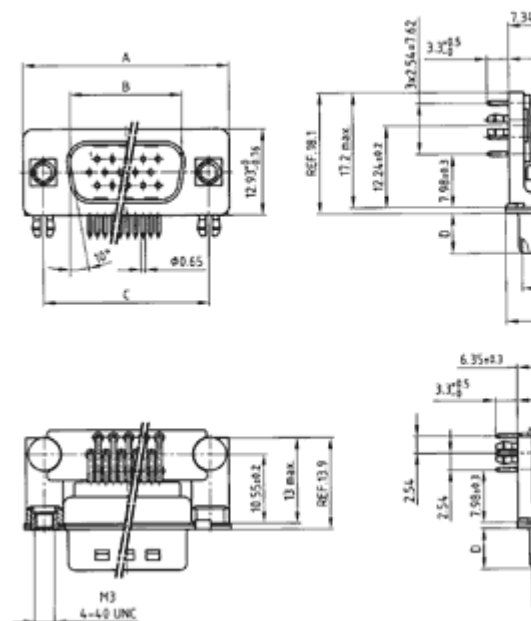
Plug connector
