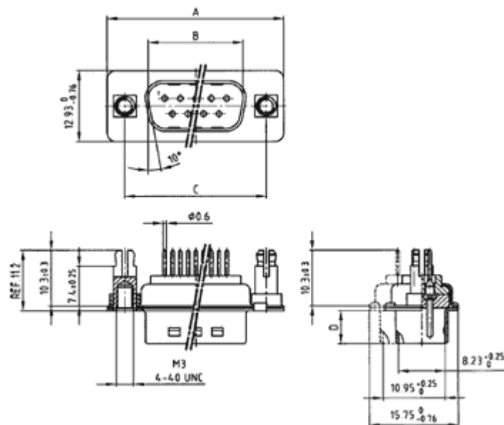
Plug connector
