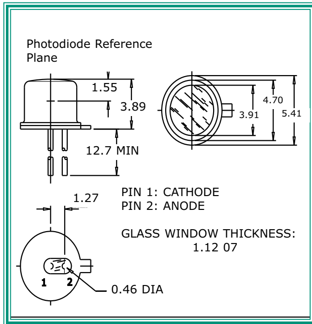
Figure 2: T0-18 Flat Window
