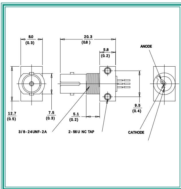
Figure 4: ST Receptacle Package
