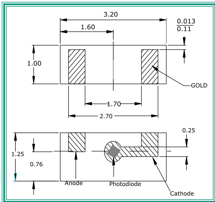
Figure 1: Ceramic Submount
