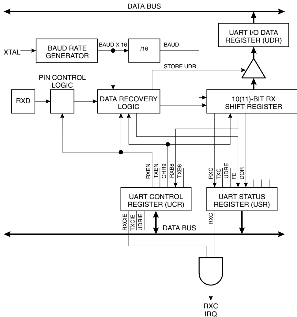
Figure 42. UART Receiver
