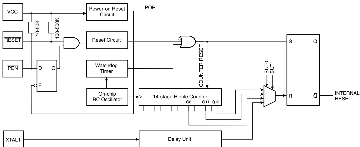
Figure 23. Reset Logic
