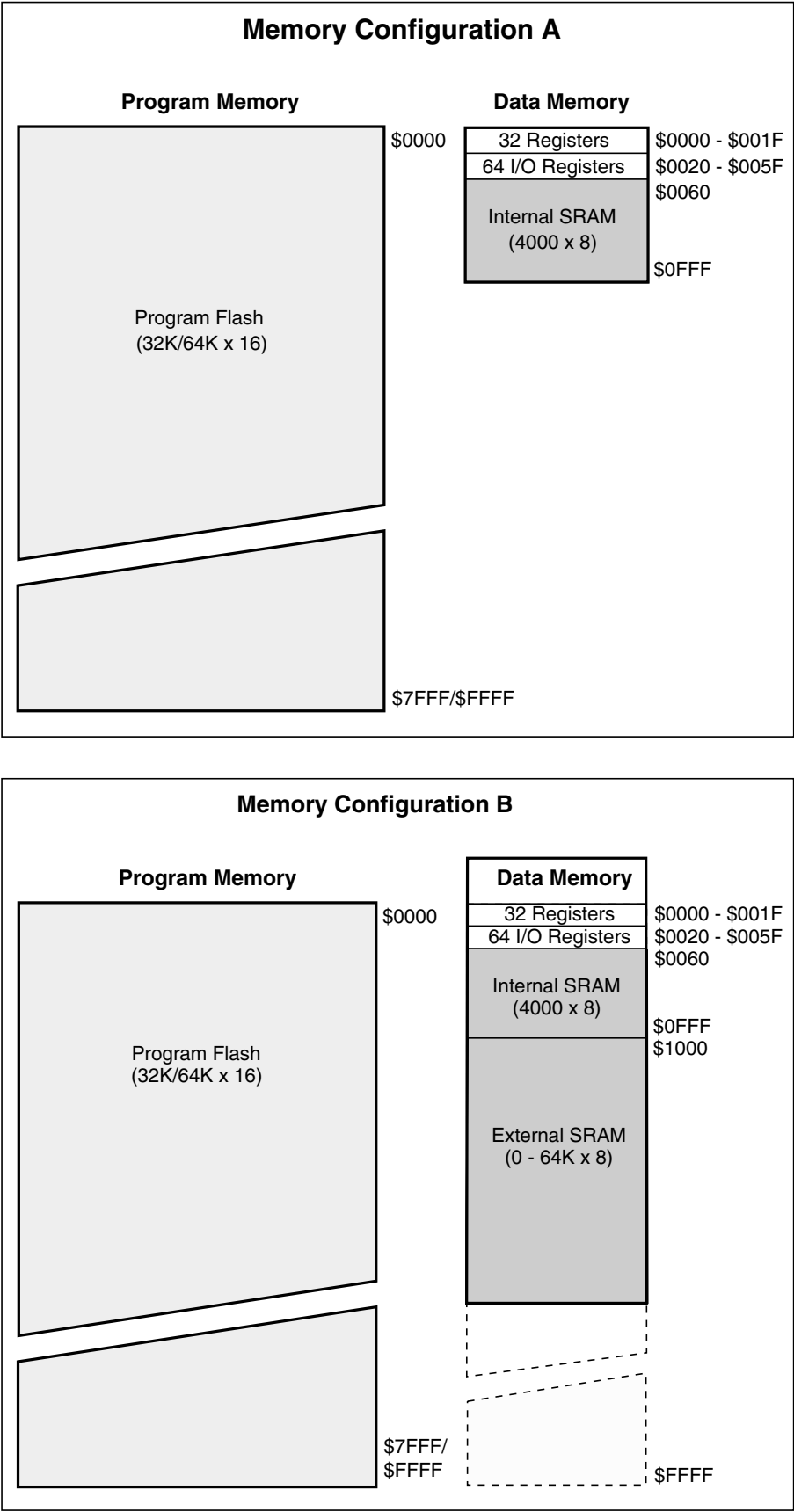
Figure 7. Memory Configurations
