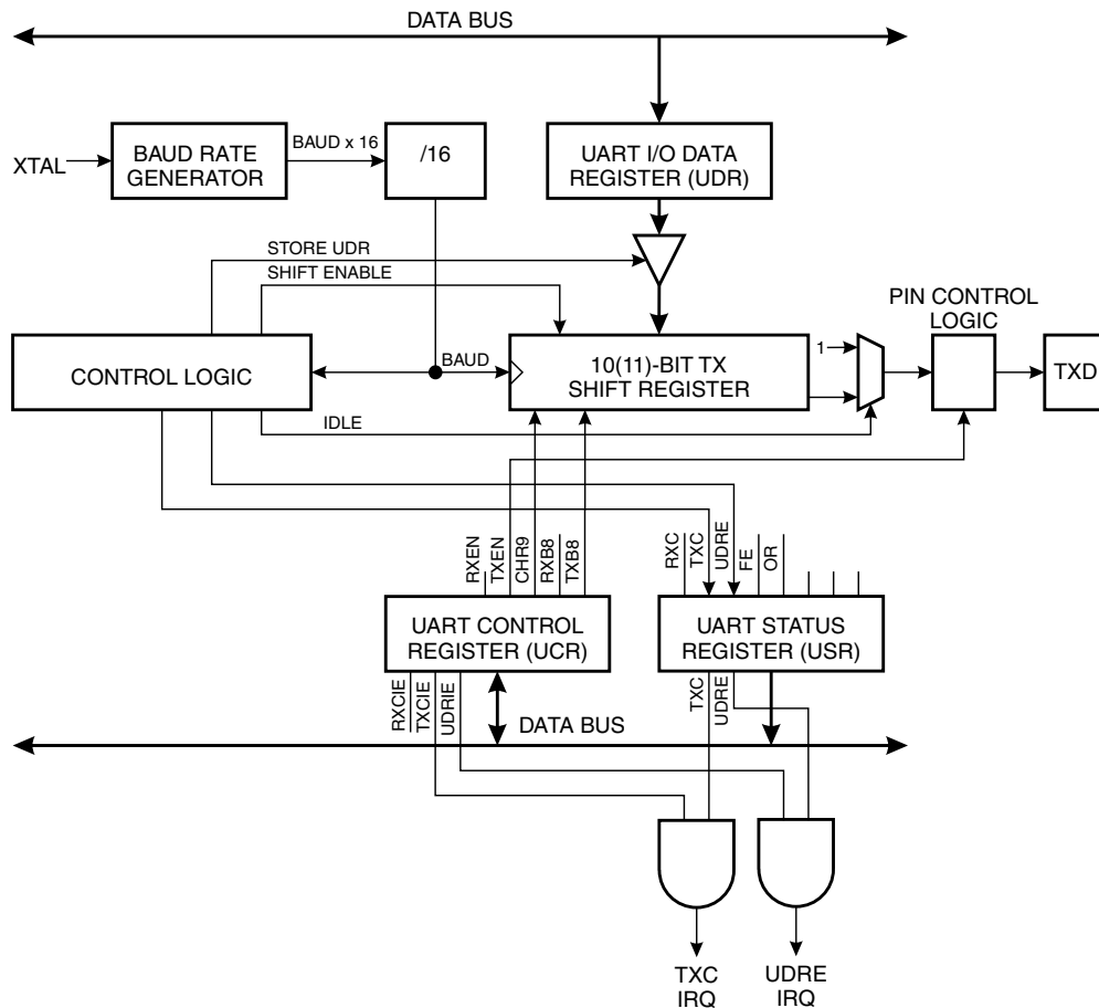
Figure 41. UART Transmitter
