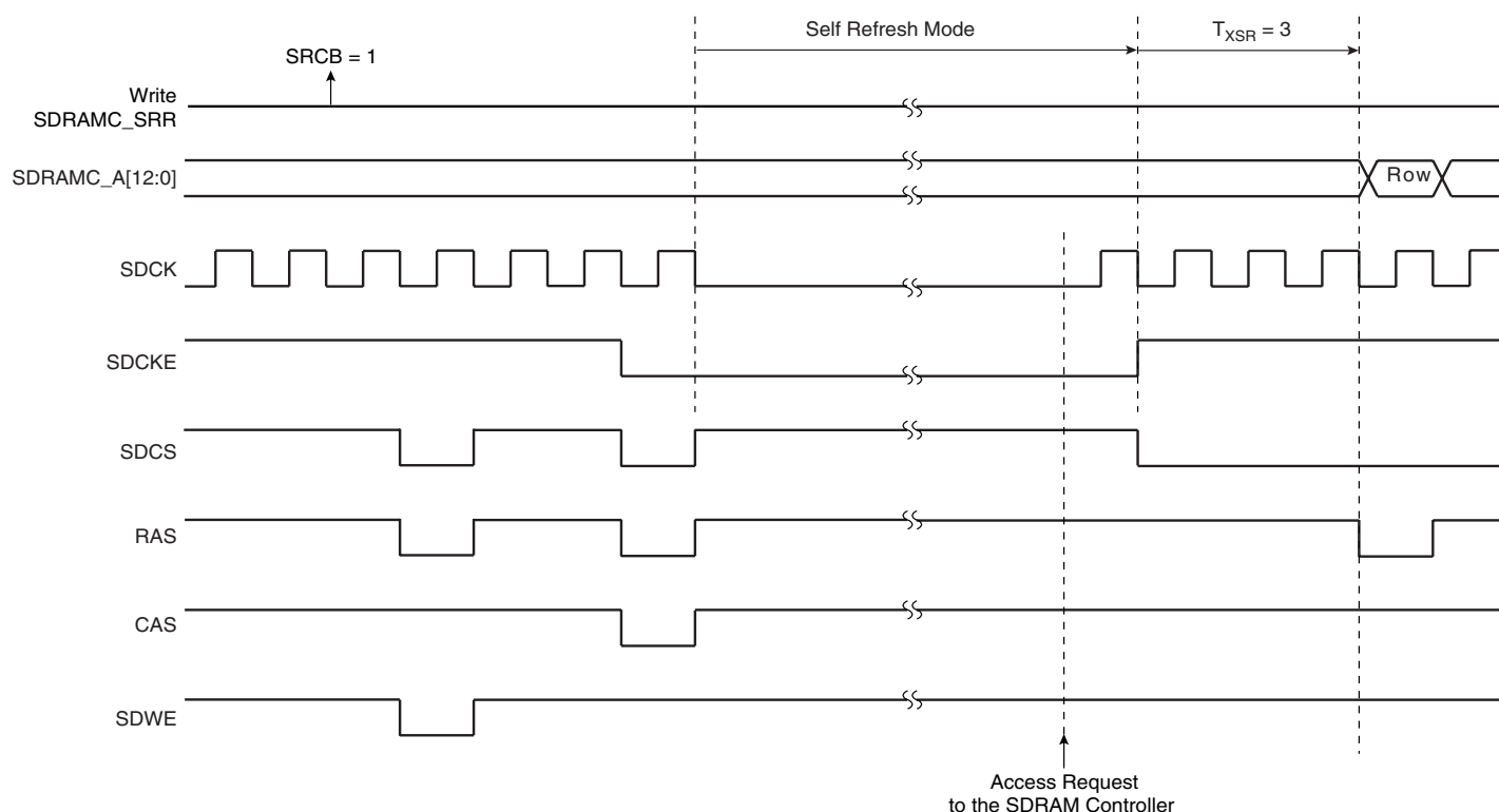
Figure 22-7. Self-refresh Mode Behavior
