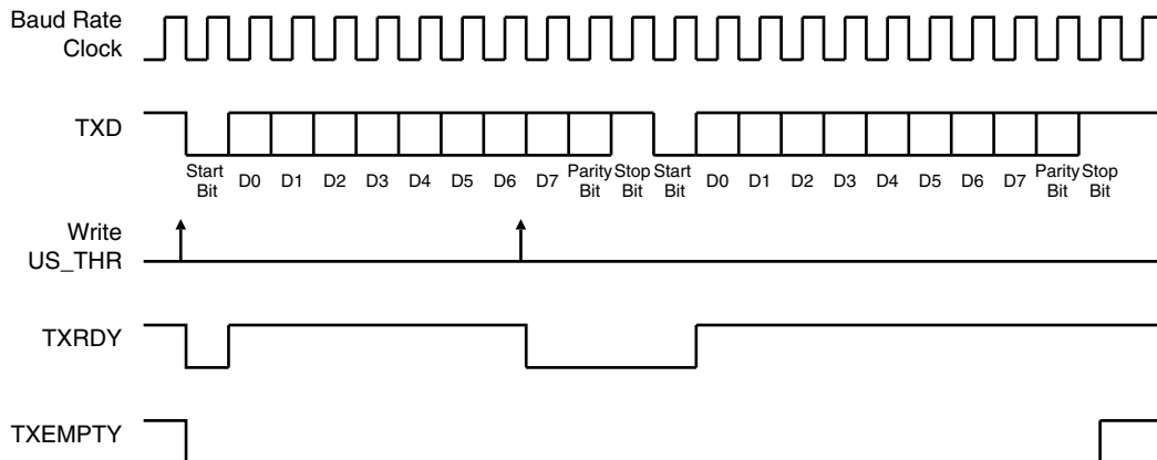
Figure 31-6. Transmitter Status
