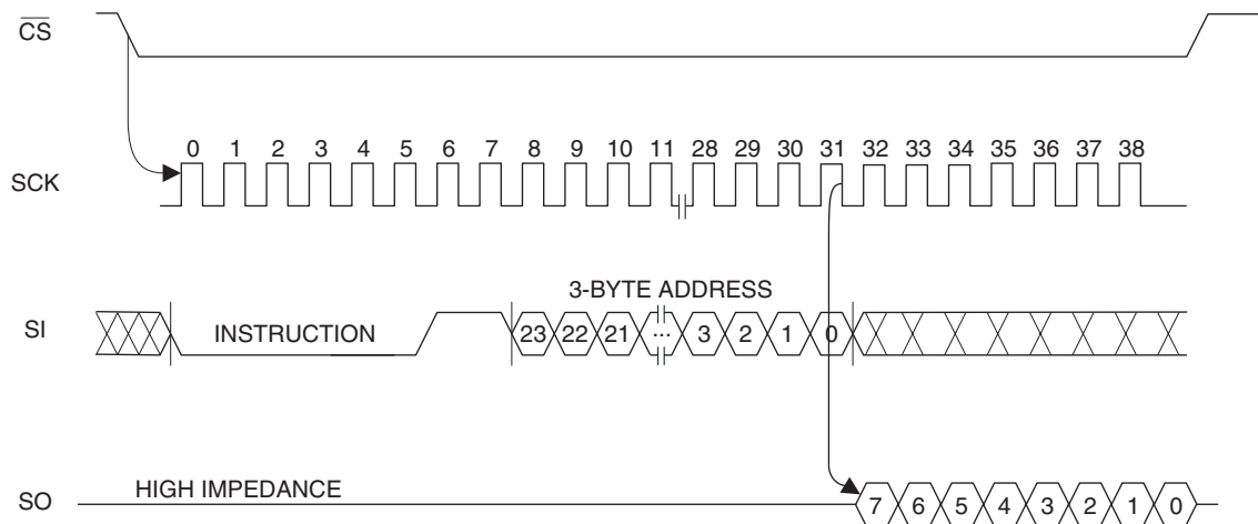
Figure 8. READ Timing
