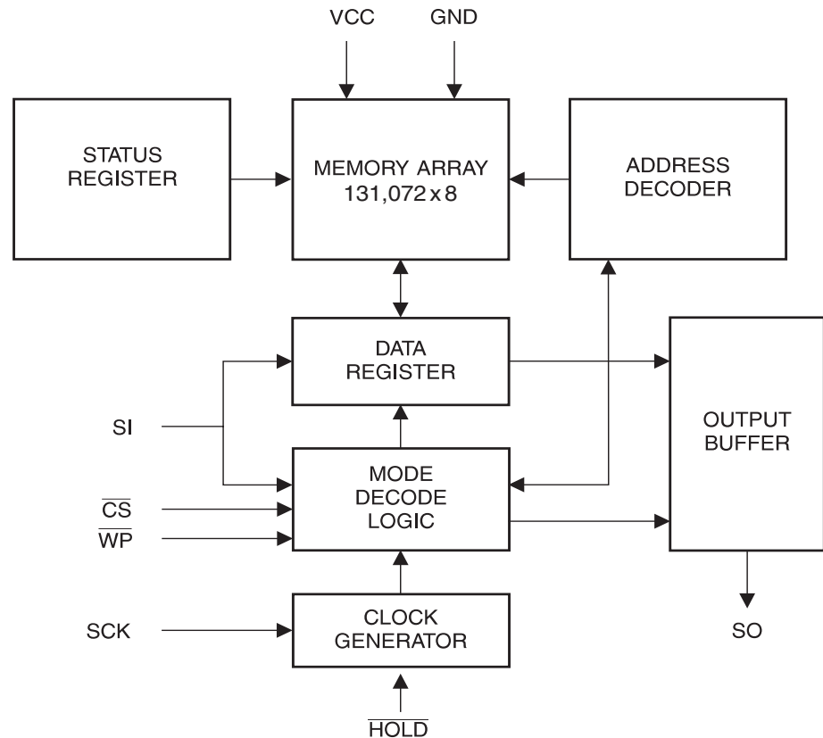
Figure 1. Block Diagram
