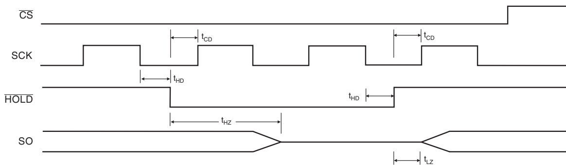
Figure 10. HOLD Timing
