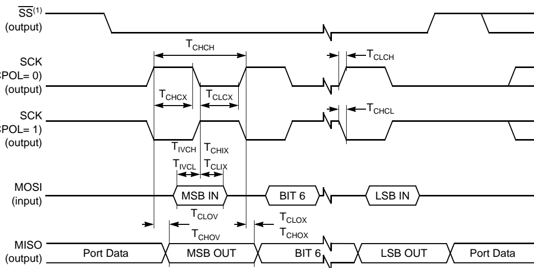
Figure 87. SPI Master Waveforms (SSCPHA= 1)
